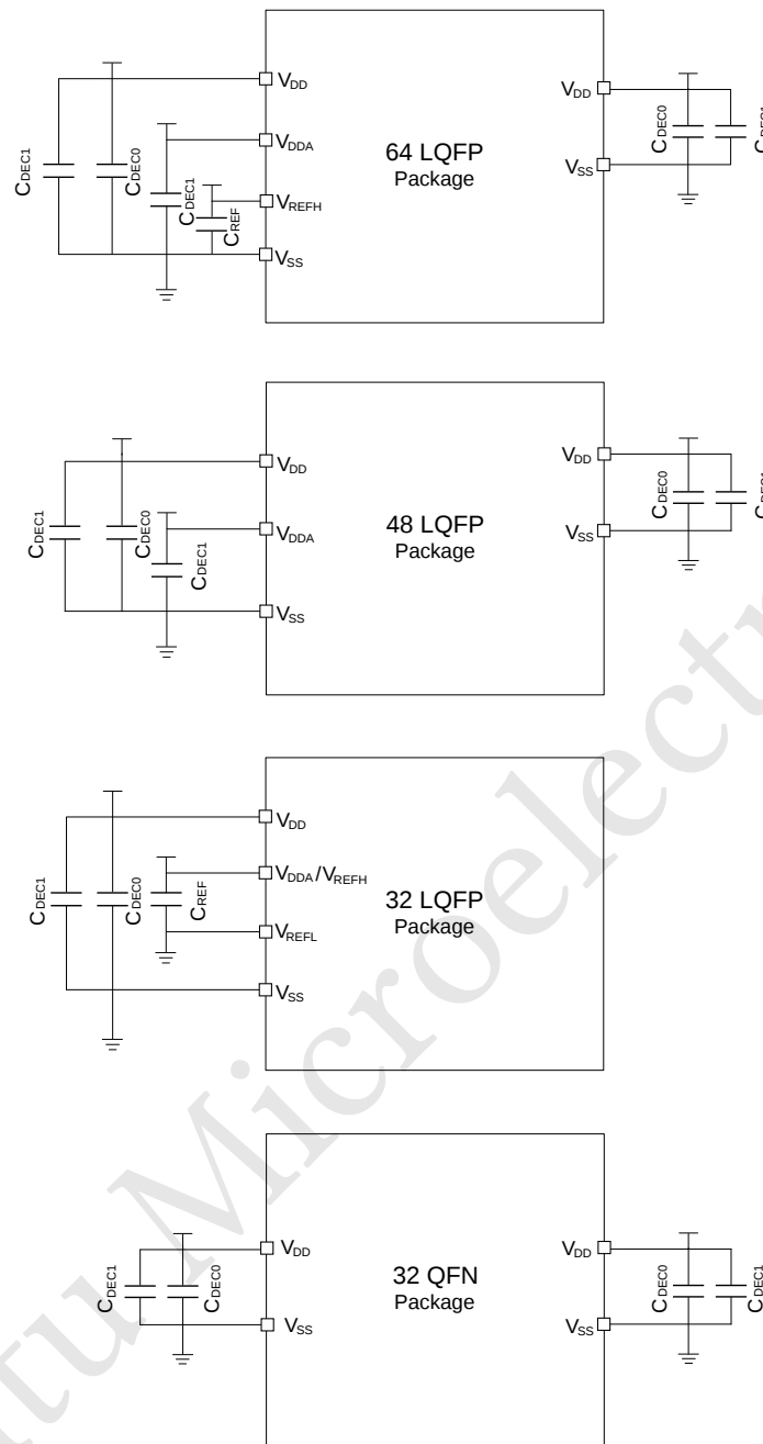
Figure 3: Pinout Decoupling
