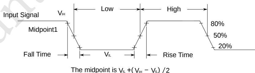
Figure 7: Input Signal Measurement Reference
