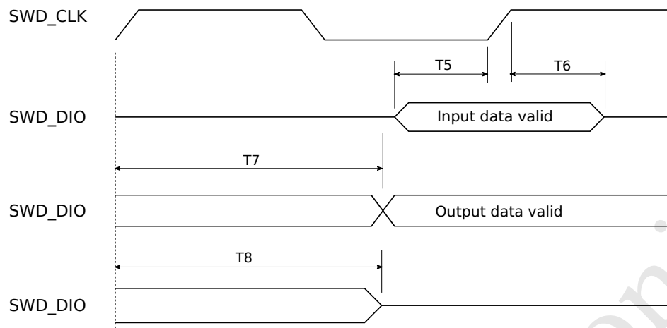
Figure 16: SWD Data Timing
