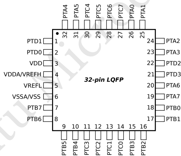
Figure 19: 32-pin LQFP Package
