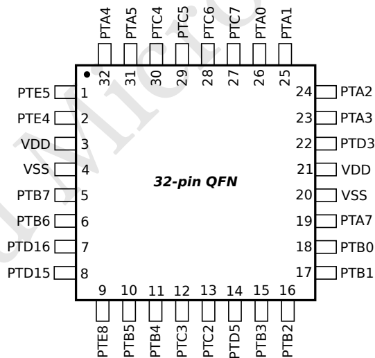
Figure 20: 32pin QFN
