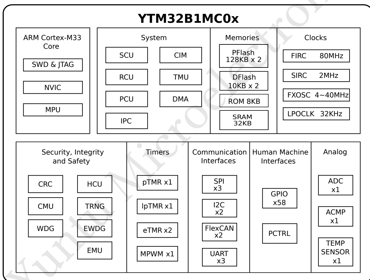
Figure 1: YTM32B1MC0x Block Diagram
