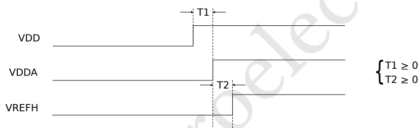
Figure 3: Power Sequence
