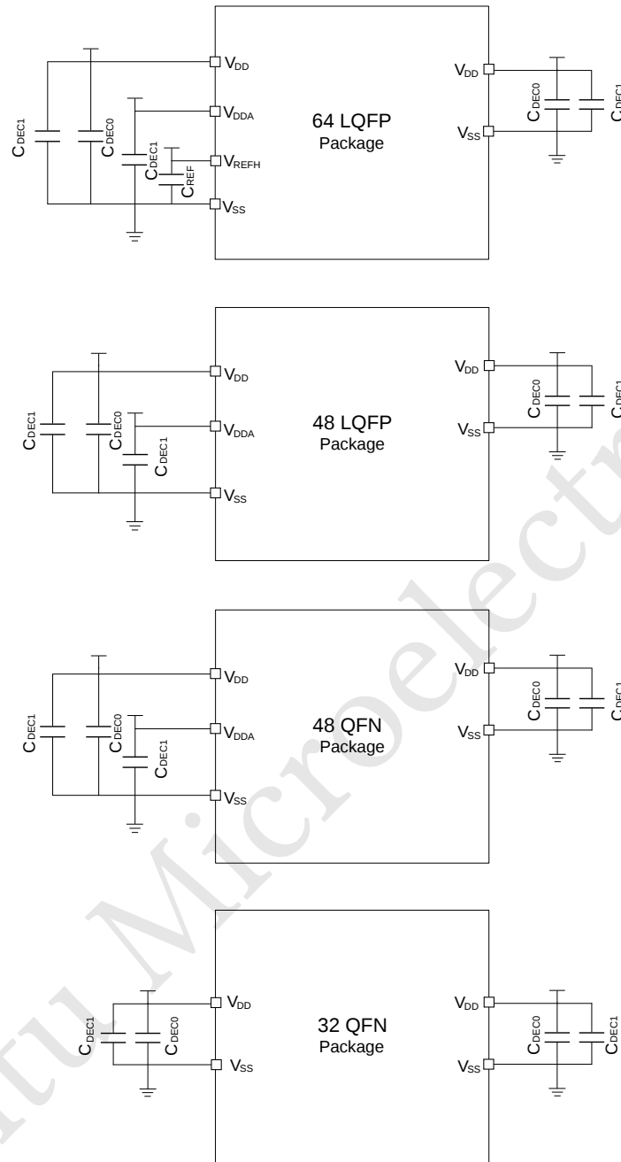
Figure 2: Pinout Decoupling
