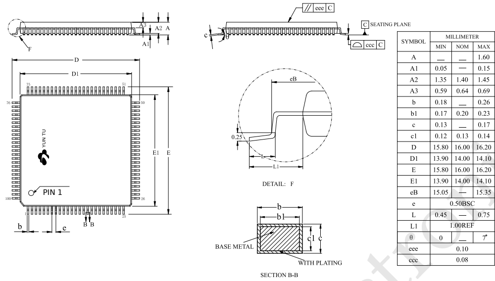
Figure 19: 100-pin LQFP
