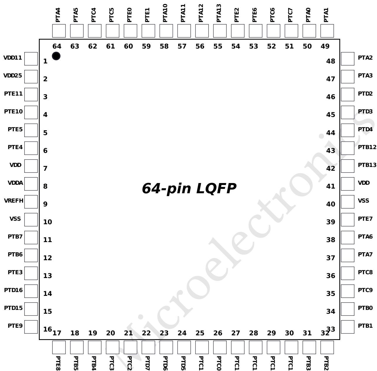
Figure 18: 64-pin LQFP Package
