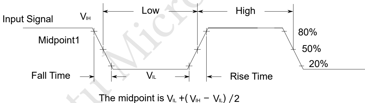
Figure 6: Input Signal Measurement Reference
