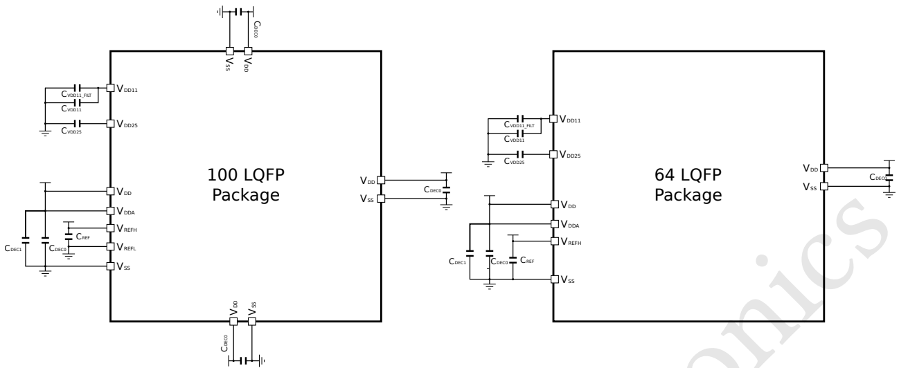
Figure 3: Pinout Decoupling
