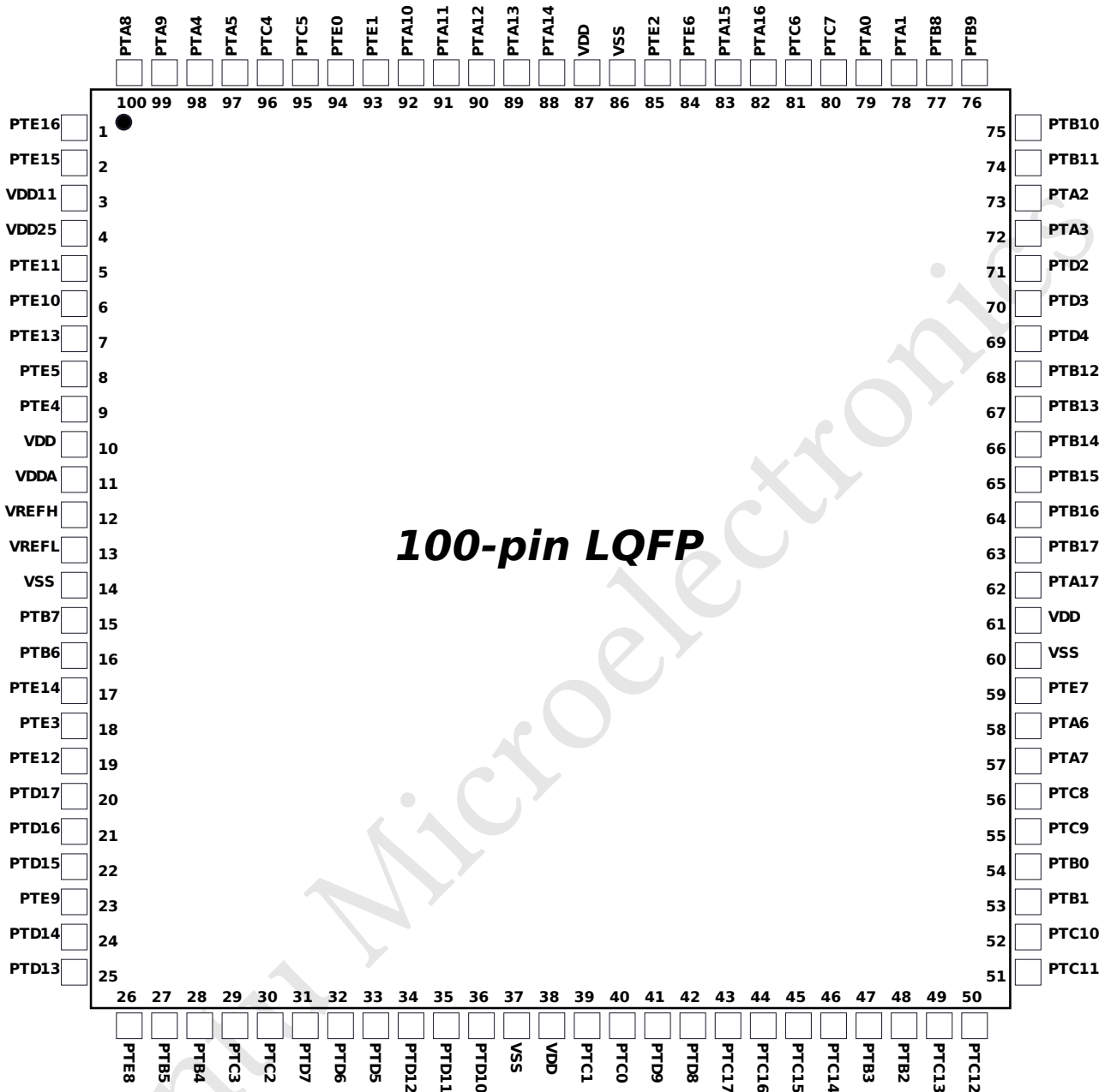
Figure 17: 100-pin LQFP Package
