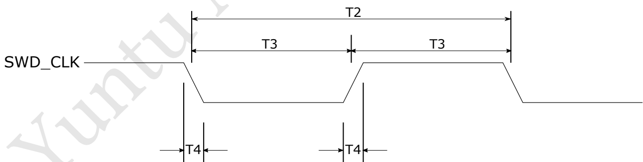
Figure 13: SWD Clock Timing
