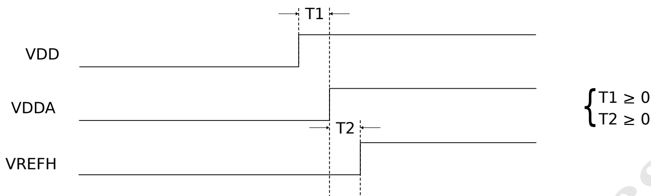
Figure 4: Power Sequence
