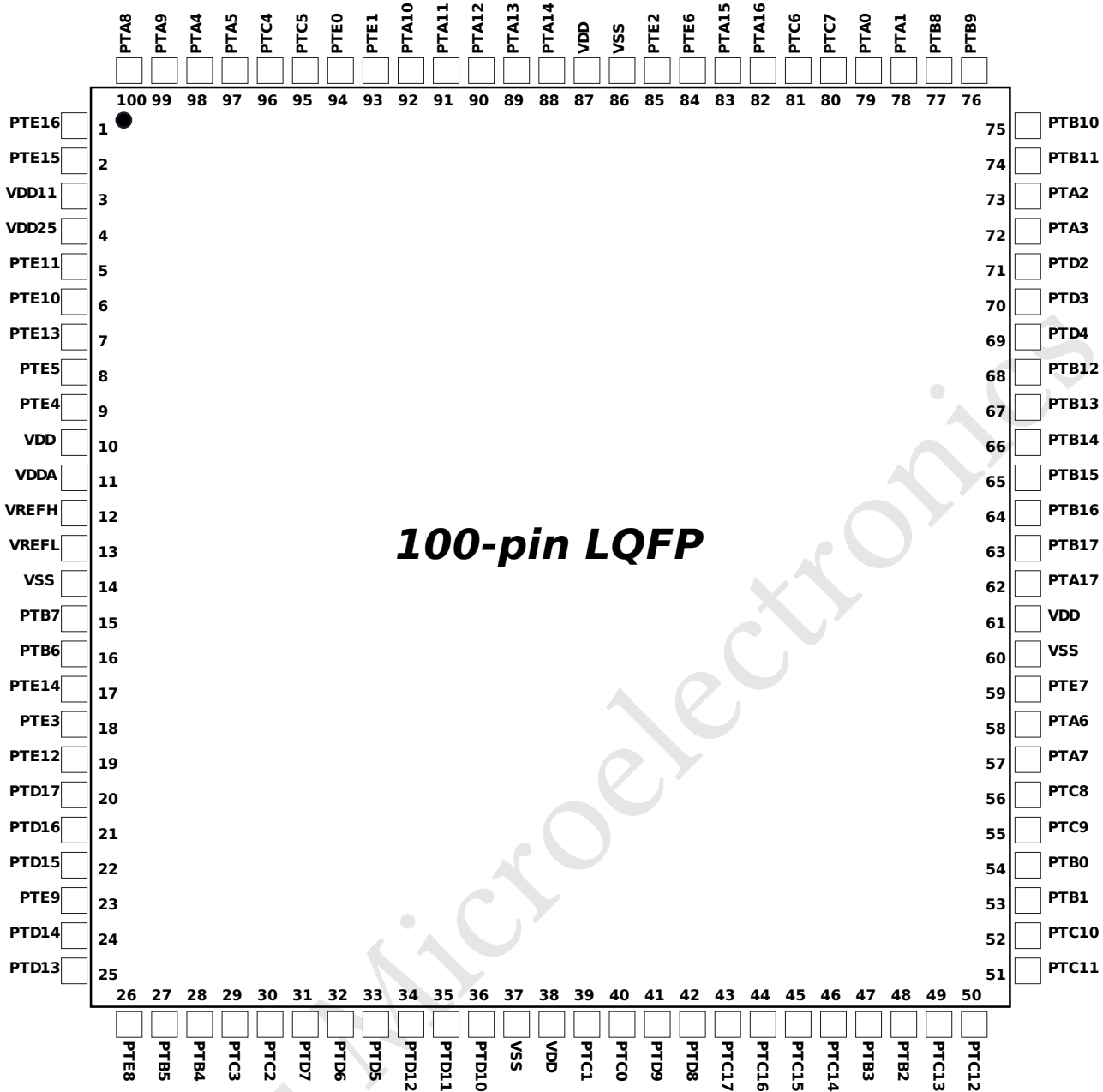
Figure 19: 100-pin LQFP Package
