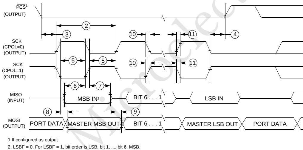
Figure 11: SPI Master Mode Timing (CHPA=1)
