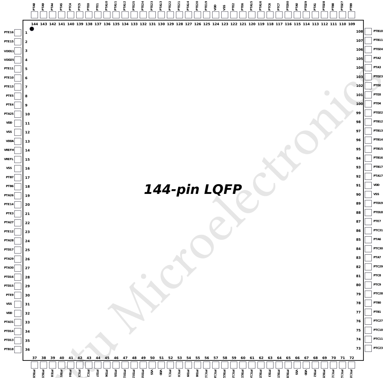
Figure 18: 144-pin LQFP Package
