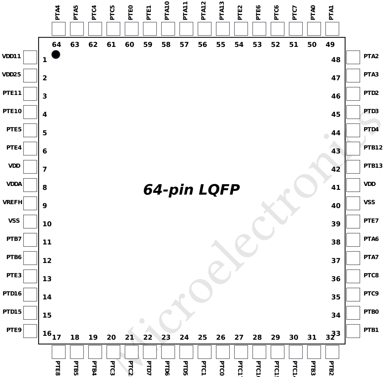
Figure 20: 64-pin LQFP Package
