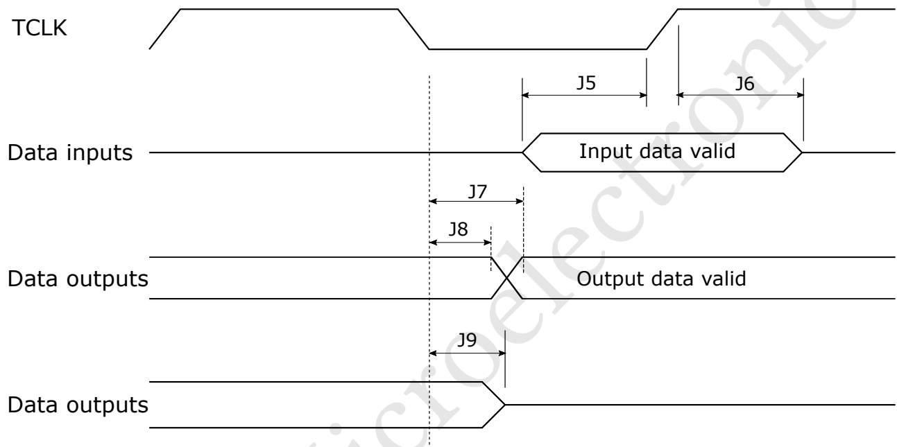
Figure 17: JTAG Data Timing
