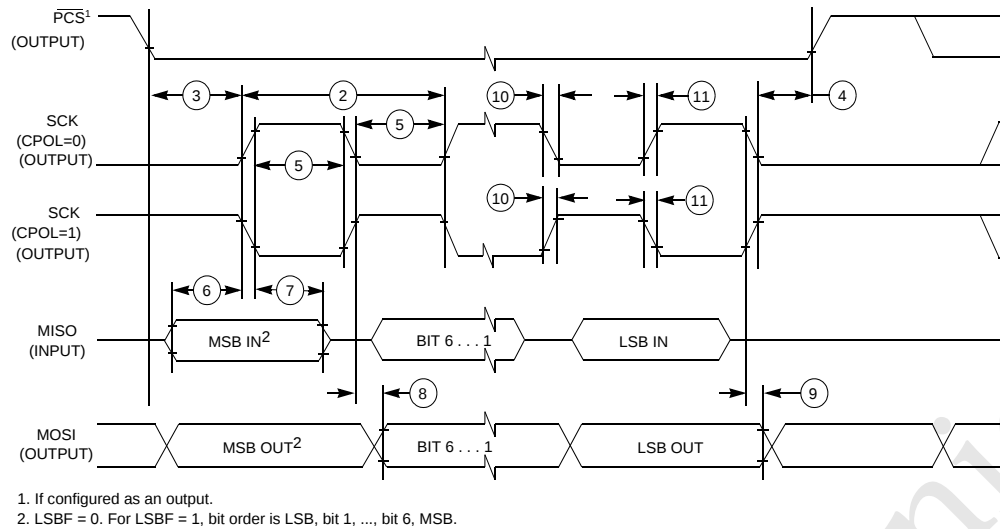
Figure 10: SPI Master Mode Timing (CHPA=0)
