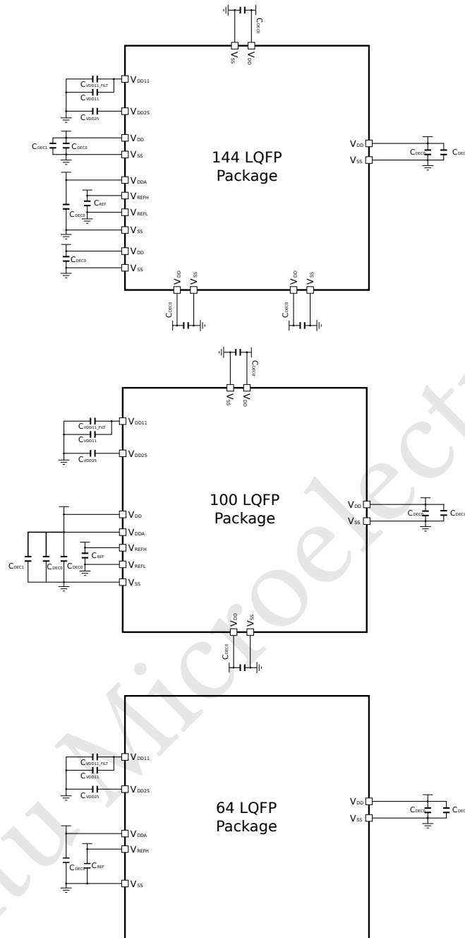
Figure 3: Pinout Decoupling
