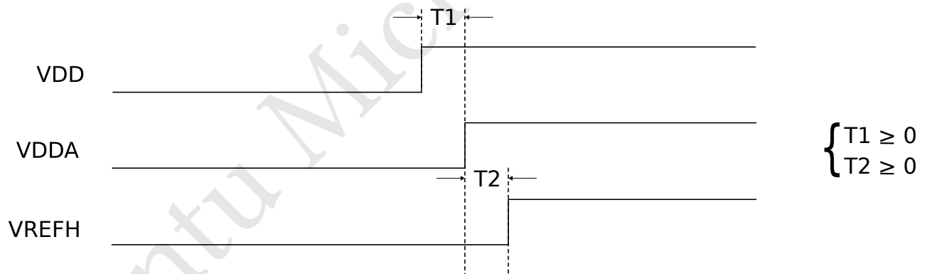
Figure 4: Power Sequence
